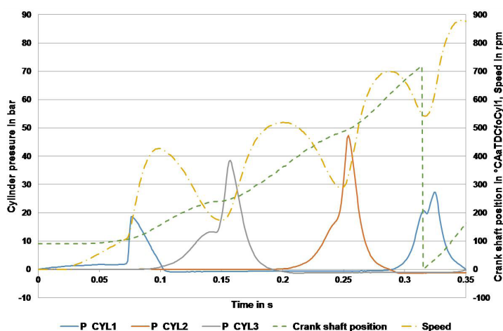
Fig 1: Conventional directstart with air injection into cylinder 1
